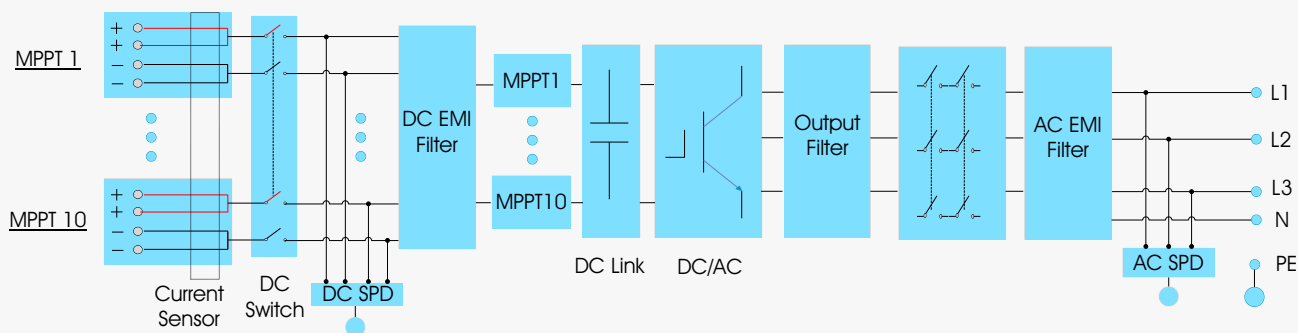
Topology Diagram
