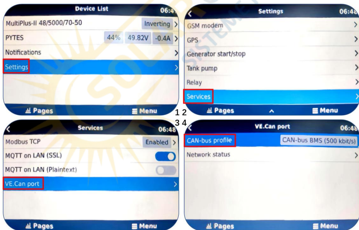
Figure 2.1.3.8 CAN-Port Setting
