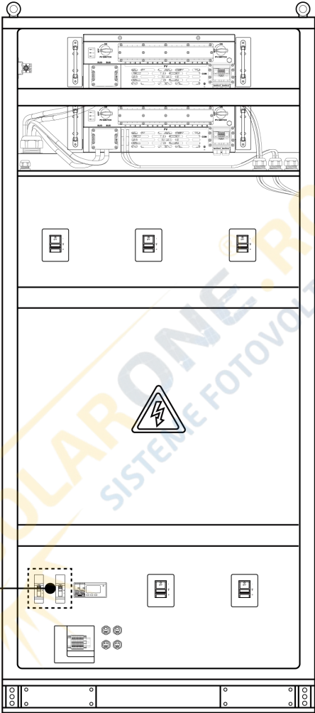
MPPT1 DC Breaker MPPT2 DC Breaker
