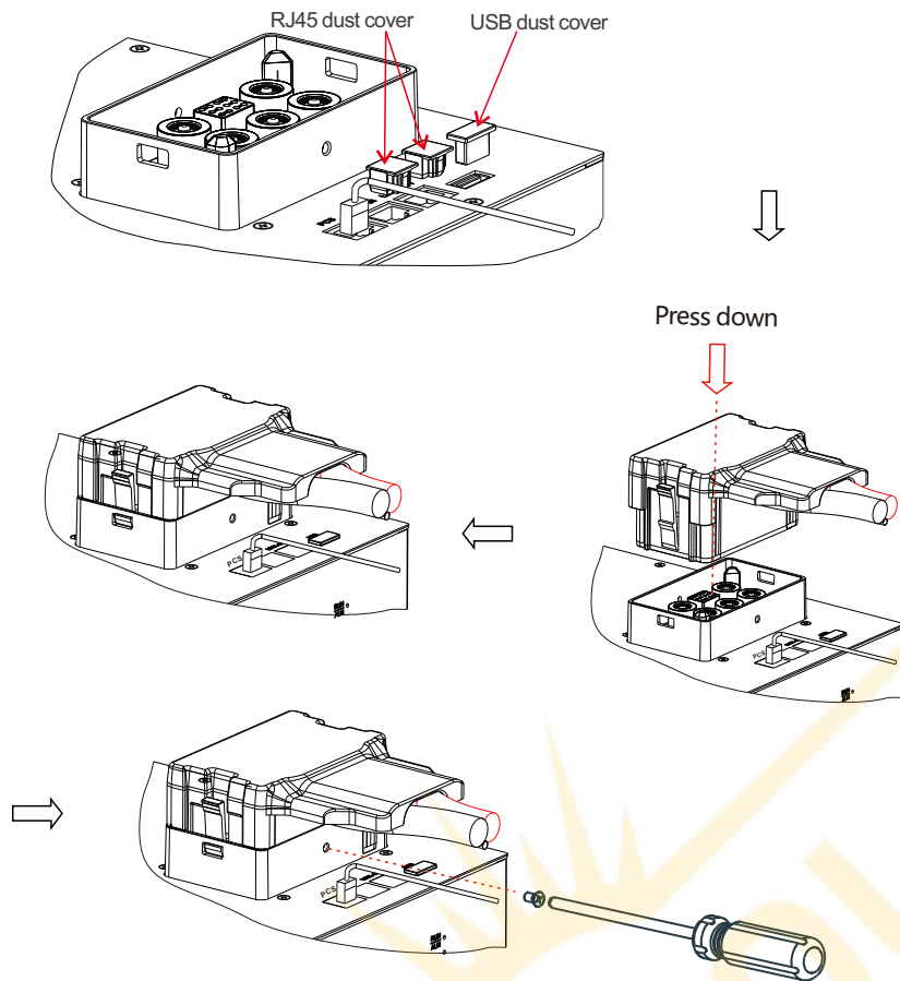
Fig 4.8: Power connection
