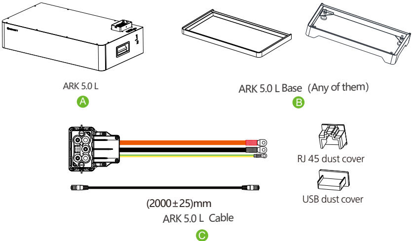
Fig 4.4: Parts list
