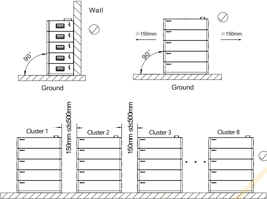
Ground(2~8 clusters installation) Fig 4.2: Acceptable floor standing installation
