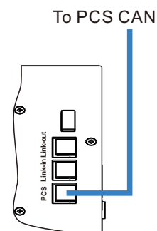
Fig 4.7: Single cluster communication wiring
