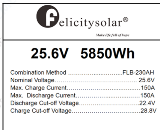
电池铭牌(含 Wh) Battery nameplate (With Wh)
